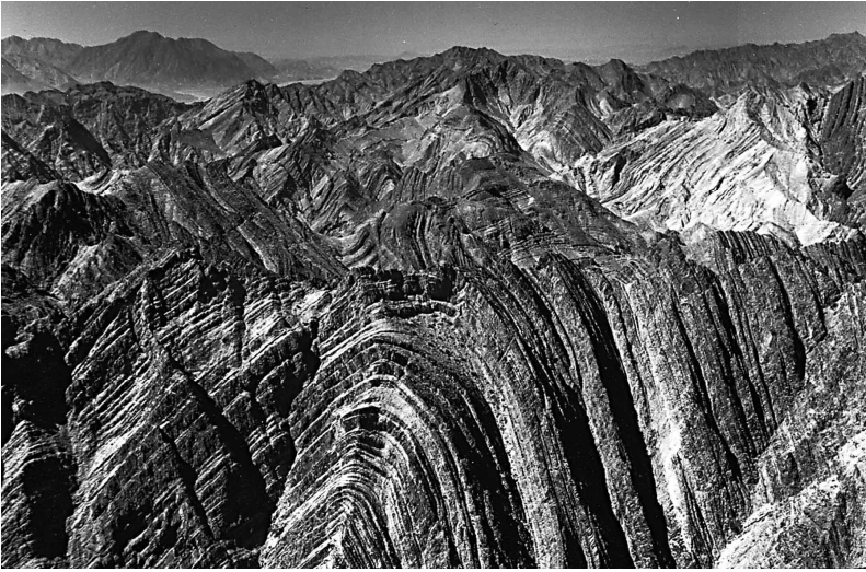
Folded mountains
