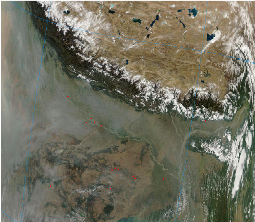
Continental-continental convergence
