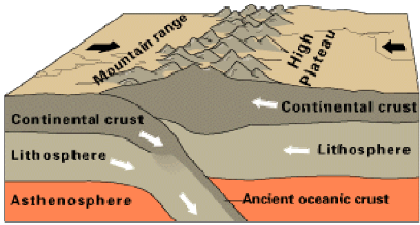
Continental-continental convergence
