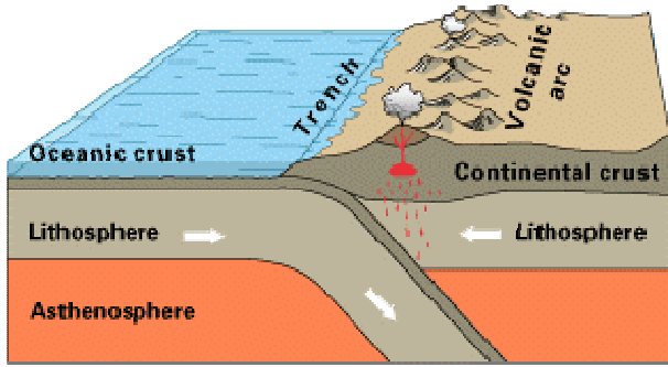
Oceanic-continental convergence
