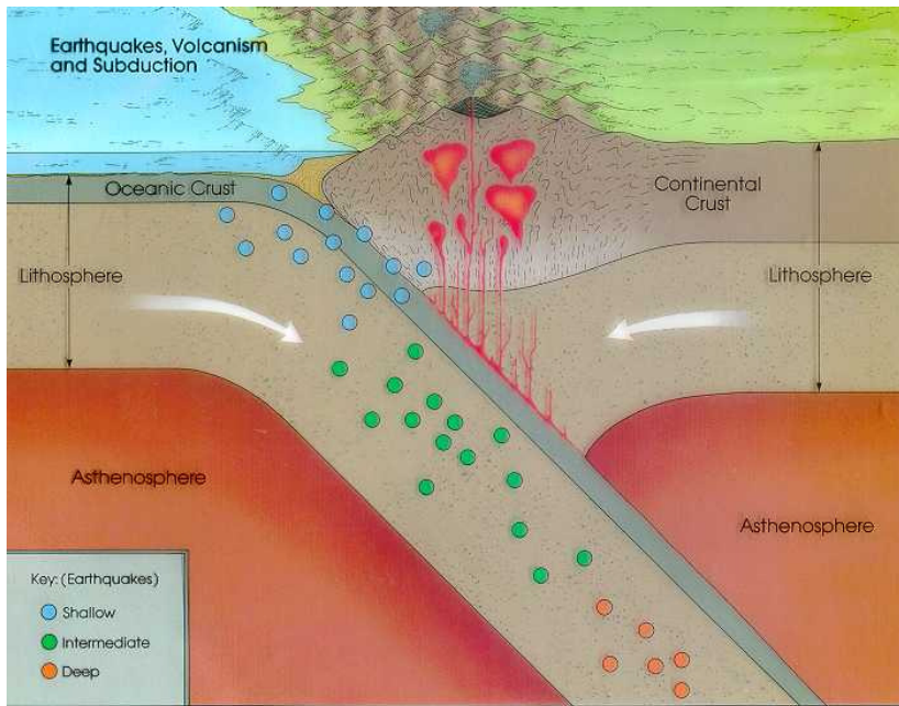
Oceanic-continental convergence
