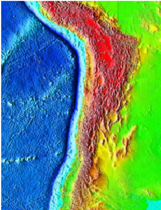
South American Trench
