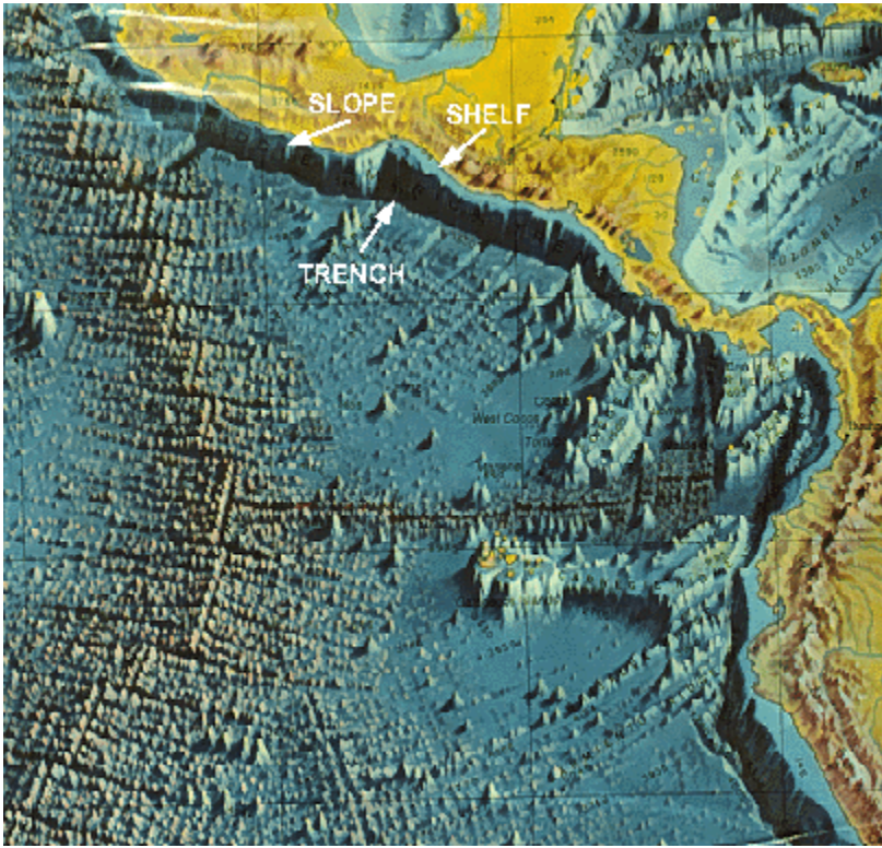
Trench off the west coast of Central America
