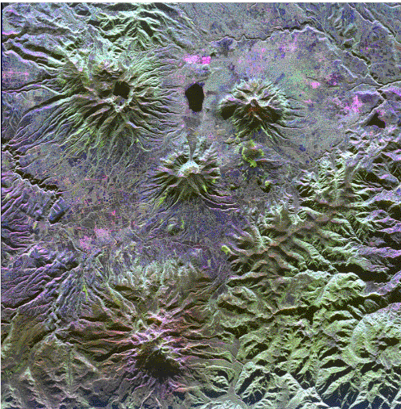
Andes Volcanoes in Ecuador from space
