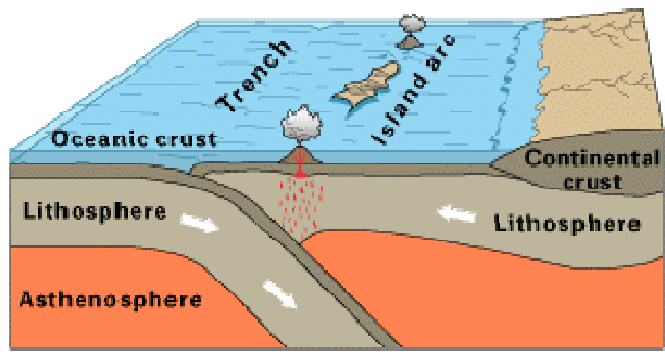
Oceanic-oceanic convergence
