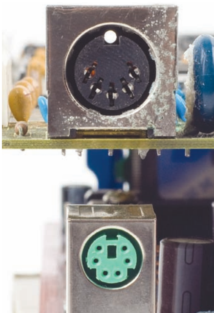
• Figure 3.9 DIN (top) and mini-DIN (bottom) connectors
