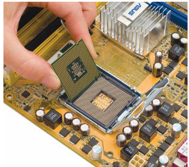
• Figure 3.37 CPU and matching socket
