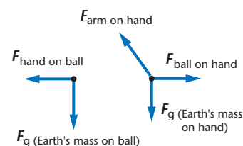
FIGURE 6–13 In addition to the external forces on the two systems, there are forces of interaction between the hand and the ball.
