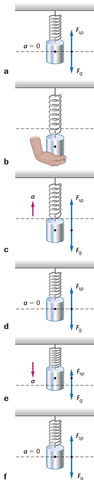
FIGURE 6–10 Simple harmonic motion is demonstrated by the vibration of a block hanging on a spring.
