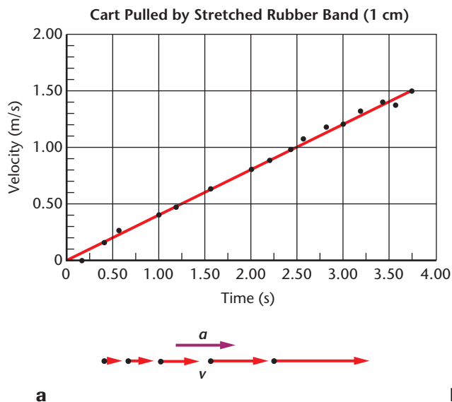
FIGURE 6-2 The constant slope of the line indicates that the acceleration of the cart is constant. The cart used in this experiment is shown in b . It is designed to minimize friction.
