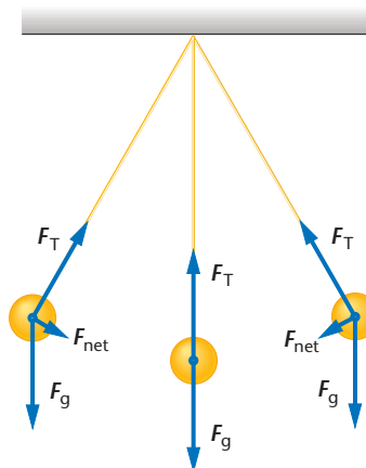
FIGURE 6–11 F_{\text{net}} , the vector sum of F_T and F_g , is the restoring force of the pendulum.
