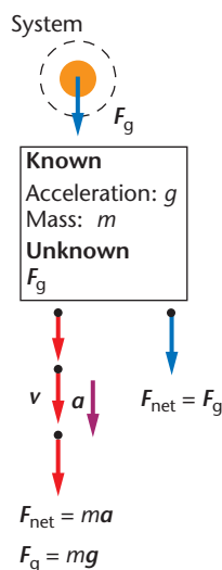
FIGURE 6–5 The net force on the ball is the weight force, F_g .
