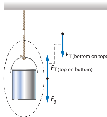
FIGURE 6–15 The tension in the rope is equal to the weight of all objects hanging from it.
