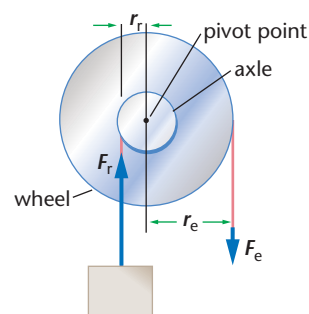
FIGURE 10-10 For levers and wheel and axles, the IMA is r_e/r_r .
