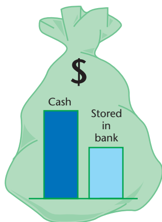
FIGURE 11-4 Money in the bank and cash in your pocket are different forms of the same thing.
