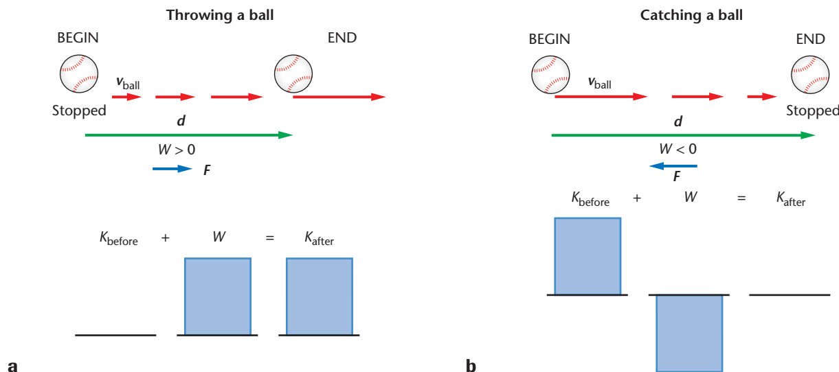
FIGURE 11–2 When you throw a ball, you do work on it. The ball gains kinetic energy as a result (a) . When you catch a ball, it stops because you exert a force on it in the opposite direction from its motion (b) .
