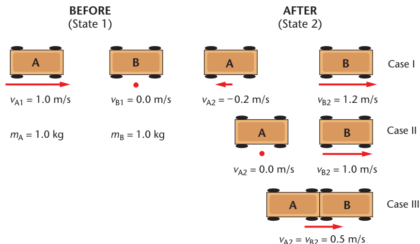
FIGURE 11–11 The energy considerations in these three kinds of collisions between a moving object and a stationary object are different. In Case I, the two objects move apart in opposite directions. In Case II, the moving object comes to rest, and the stationary object begins to move. In Case III, the two objects stick together and move as one.
