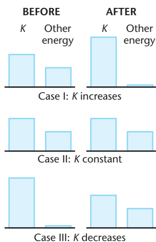
FIGURE 11–12 Bar graphs can be drawn to represent the three kinds of collisions.
