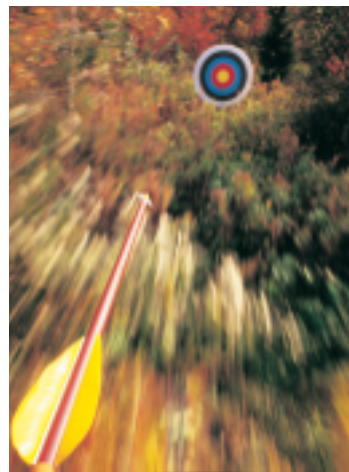
FIGURE 11-7 Elastic potential energy is stored in the string of this bow. Before the string is released, the energy is all potential. As the string is released, the energy is transferred to the arrow as kinetic energy.
