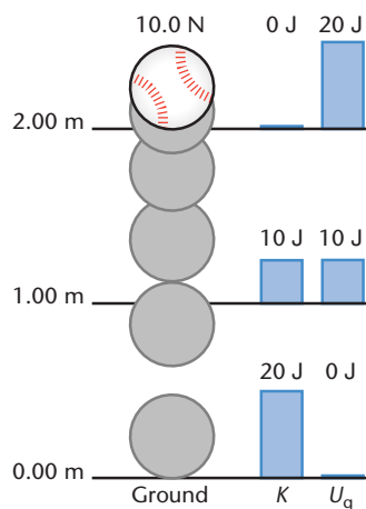
FIGURE 11-8 The decrease in potential energy is equal to the increase in kinetic energy.
