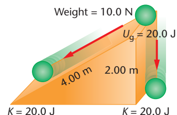
FIGURE 11–9 The path an object follows in reaching the ground does not affect the final kinetic energy of the object.
