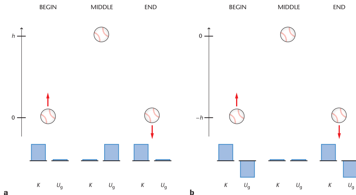
FIGURE 11–6 The energy of a ball is converted from one form to another in various stages of its flight (a) . Note that the choice of a reference level is arbitrary but that the total energy remains constant (b) .
