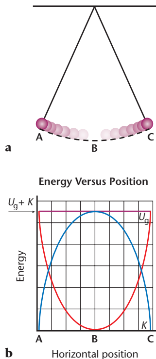
FIGURE 11-10 For the simple harmonic motion of a pendulum bob (a), the mechanical energy—the sum of the potential and kinetic energies—is a constant (b).
