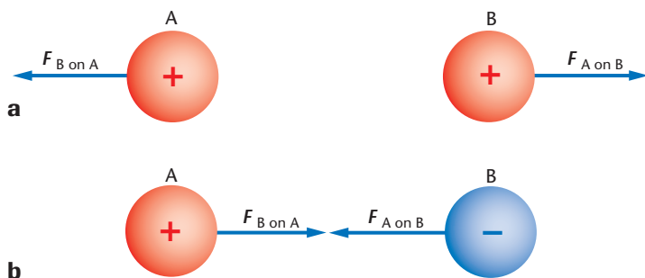
FIGURE 20-11 The rule for determining direction of force is like charges repel, unlike charges attract.
