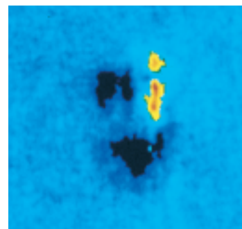
FIGURE 20–4 A piece of plastic 0.02 mm wide was given a net positive charge. Areas of negative charge are visible as dark regions. Areas of positive charge are visible as yellow regions.
