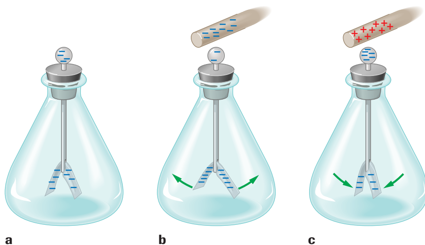
FIGURE 20–8 A negatively charged electroscope will have its leaves spread (a) . A negatively charged rod pushes electrons down to the leaves, causing them to spread more (b) . A positively charged rod attracts some of the electrons from the leaves, causing them to spread apart less (c) .
