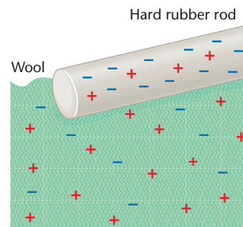
FIGURE 20–3 As the rubber rod strokes the wool, electrons are removed from the wool atoms and cling to the rubber atoms. In this way, both objects become charged.
