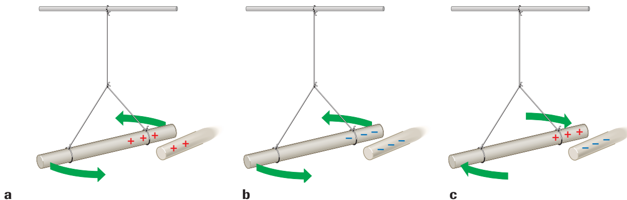
FIGURE 20–6 A charged rod, when brought close to another suspended rod, will attract or repel the suspended rod.
