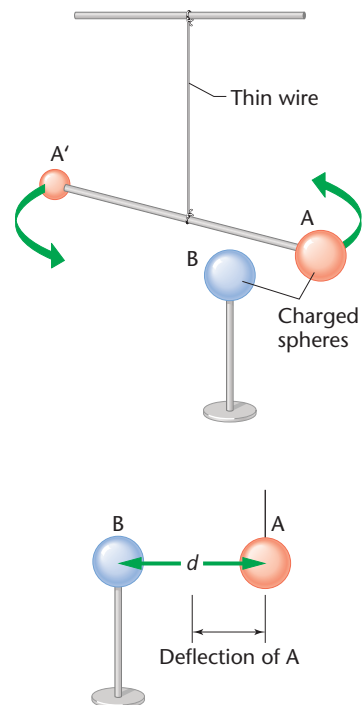
FIGURE 20–10 Coulomb used this type of apparatus to measure the force between two spheres, A and B. He observed the deflection of A while varying the distance between A and B.
