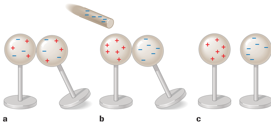
FIGURE 20–9 Start with neutral spheres that are touching (a) , bring a charged rod near them (b) , and then separate the spheres and remove the charged rod (c) . This is one example of charging by induction.
