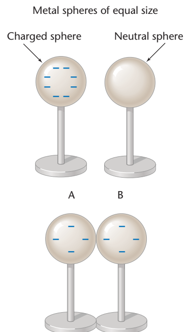
FIGURE 21–10 A charged sphere shares charge equally with a neutral sphere of equal size.
