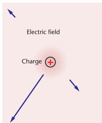
FIGURE 21-1 Arrows can be used to represent the magnitude and direction of the electric field about an electric charge at various locations.
