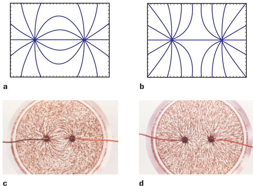
FIGURE 21-4 Lines of force between unlike charges ( a, c ) and between like charges ( b, d ) describe the behavior of a positively charged object in a field. The top photographs are computer tracings of electric field lines.
