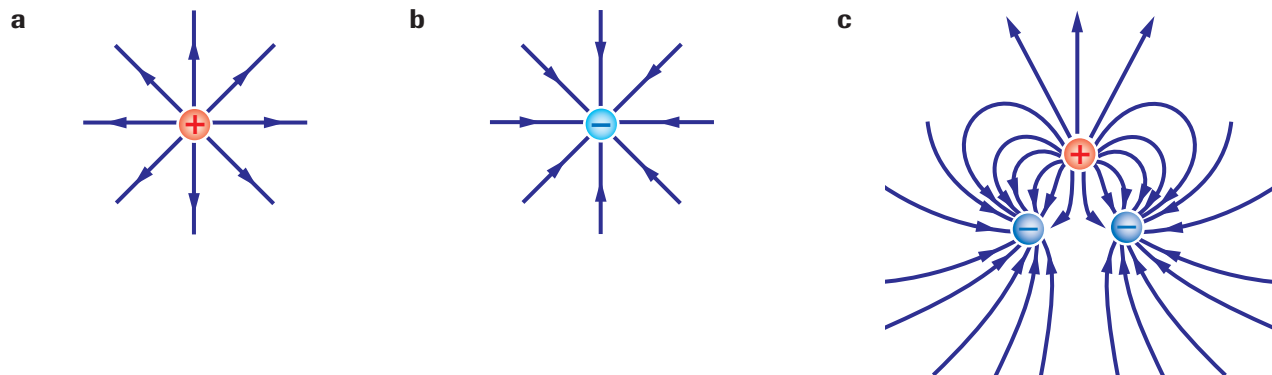
FIGURE 21-2 Lines of force are drawn perpendicularly away from the positively-charged object (a) and perpendicularly into the negatively-charged object (b) . Electric field lines between like charged and oppositely charged objects are shown in (c) .
