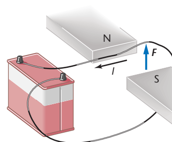
FIGURE 24–15 Current-carrying wires experience forces when they are placed in magnetic fields.
