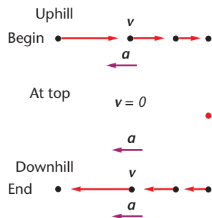
FIGURE 5-15 The acceleration of the ball is always downward.
