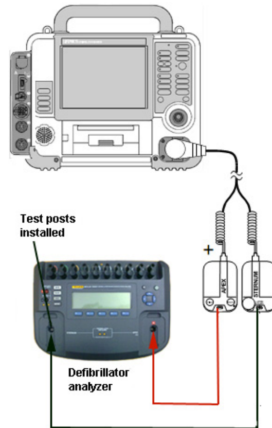
Figure 5.47—Standard paddles defibrillator delivered energy setup
