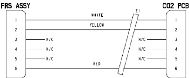
Figure 11.66—Diagram for item W30
