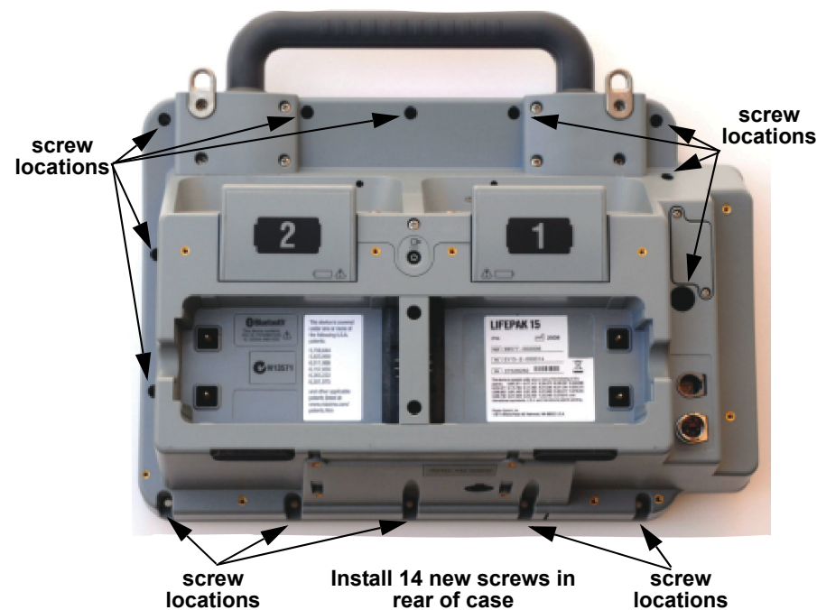
Figure 10.8—Screw locations
