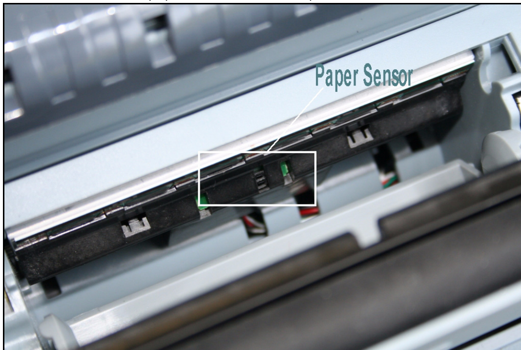
Figure 8.1—Paper sensor
