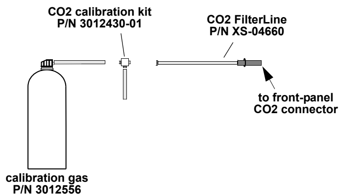
Figure 5.21—CO2 calibration connection
