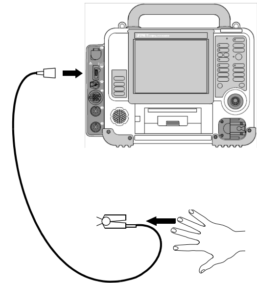
Figure 5.31—SpO2/SpCO/SpMet setup
