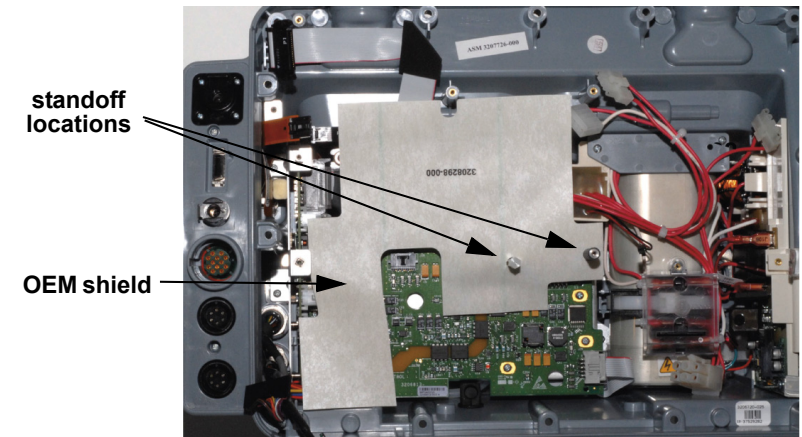
Figure 10.77—OEM shield
