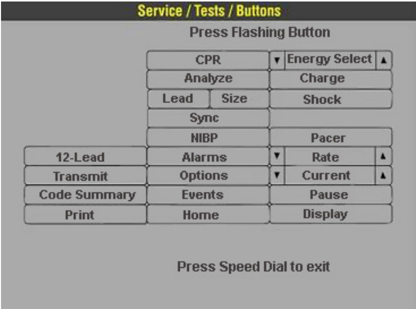
Figure 5.28—Keypad test buttons
