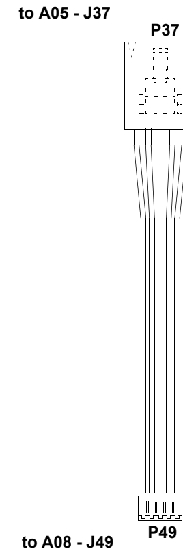
Figure 10.22—Backlight PCB/interface PCB cable connections
