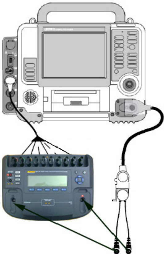
Figure 5.54—Pacer output current test setup
