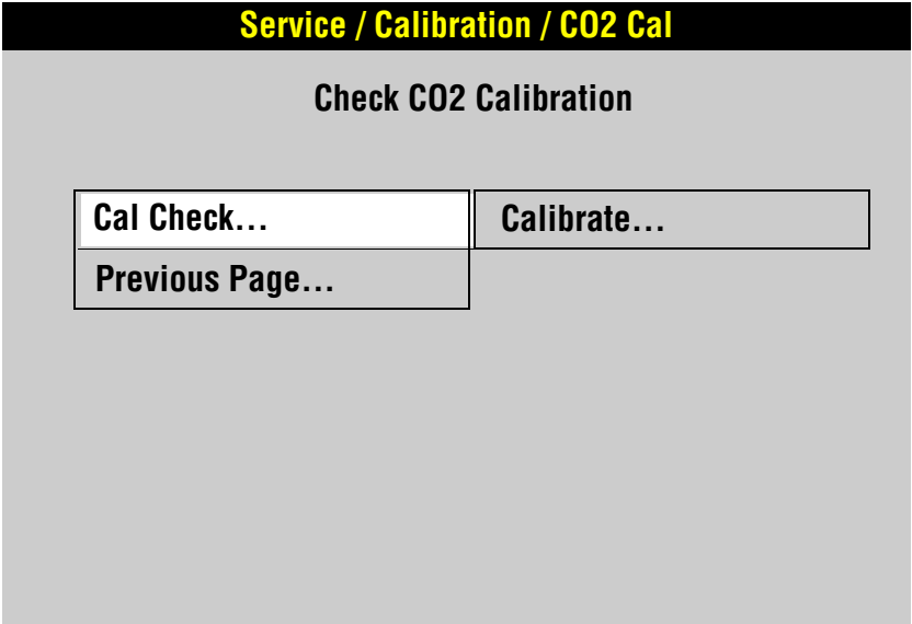
Figure 5.20—Service calibration Cal Check
