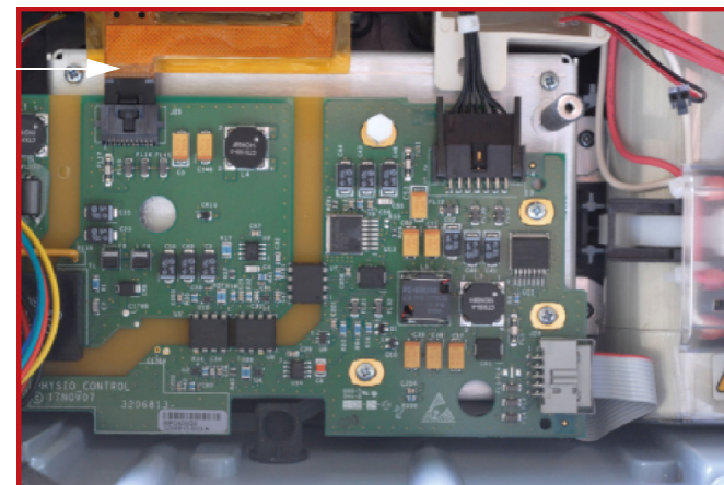
Figure 10.74—SpO2 connection to OEM PCB
