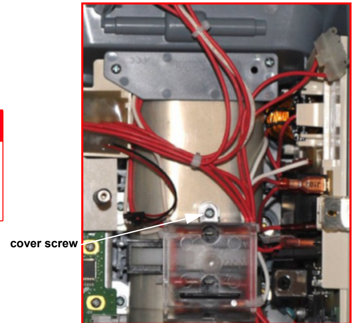
Figure 10.94—Interconnect bracket screw locations
