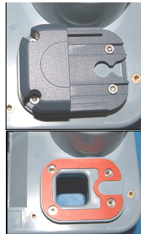
Figure 10.23—Therapy connector cable and seal
