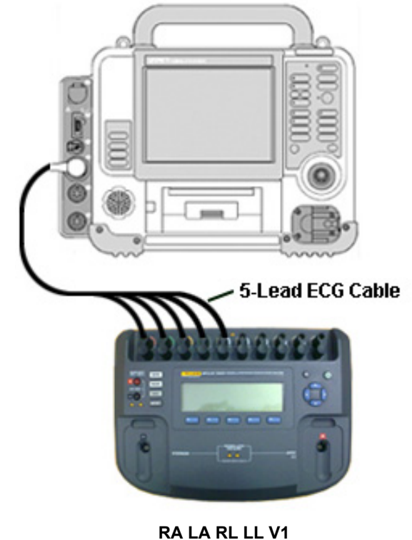
Figure 5.35—ECG 5-wire connection
