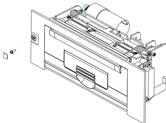
Figure 10.123—Printer assembly replacement
