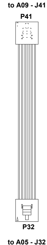
Figure 10.24—Printer control keypad/interface PCB cable connections
