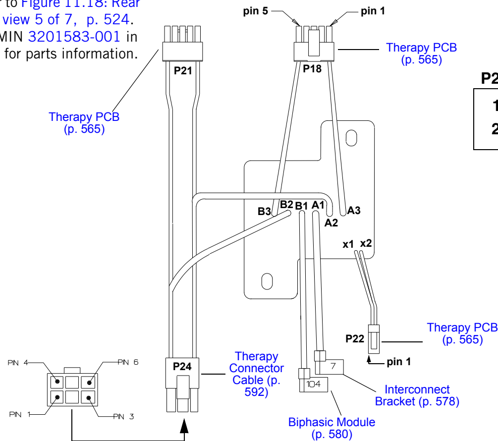
Figure 11.33—Diagram for item A13
