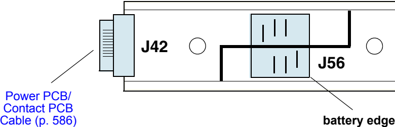
Figure 11.27—Diagram for item A07
