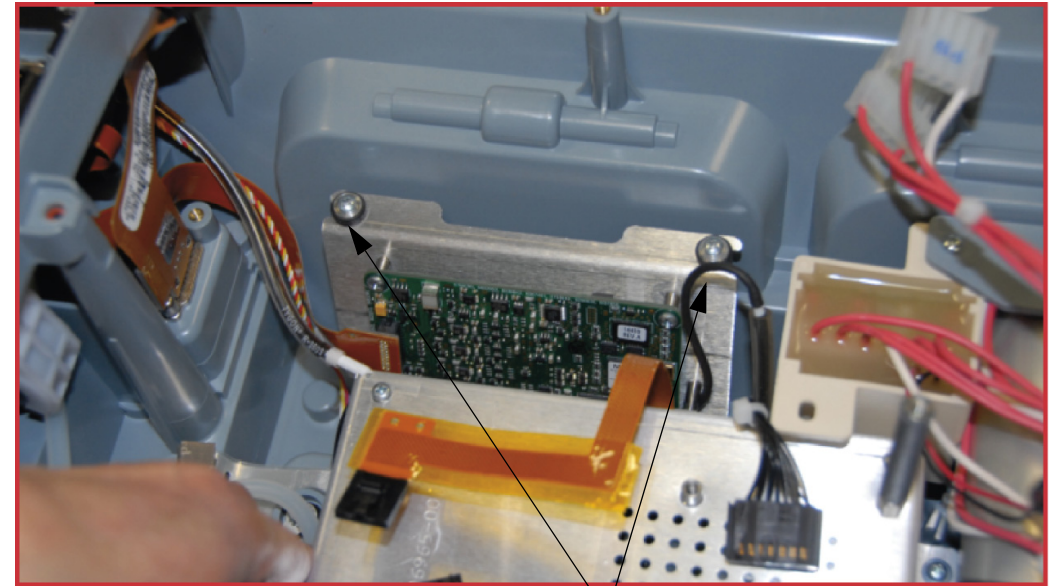
Figure 10.69—SpO2 mounting bracket
