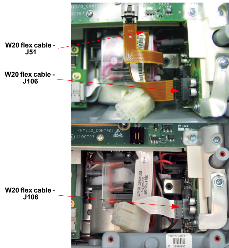
Figure 10.42—W20 flex cable connections
