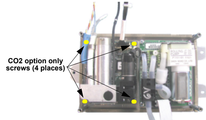
Figure 10.87—CO2 sub-assembly screw locations
