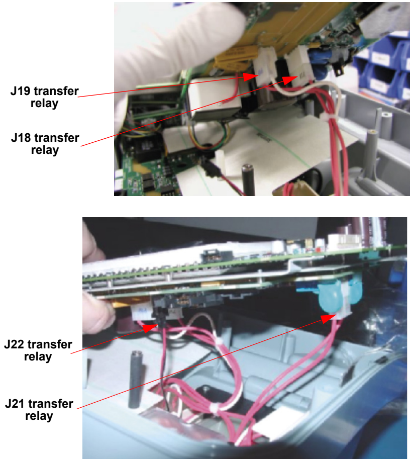
Figure 10.41—System/therapy PCB cable connections
