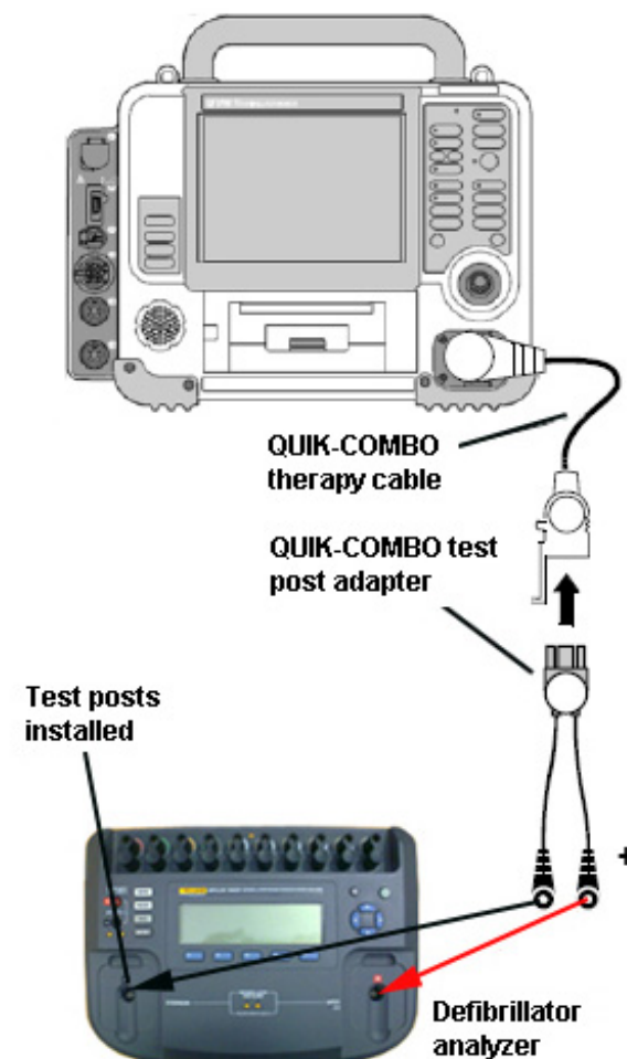
Figure 6.9—Output waveform test setup
