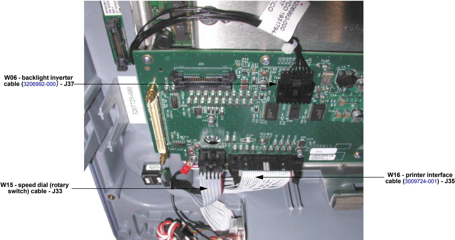
Figure 10.12—Interface PCB cable connection locations - view 2 of 2
