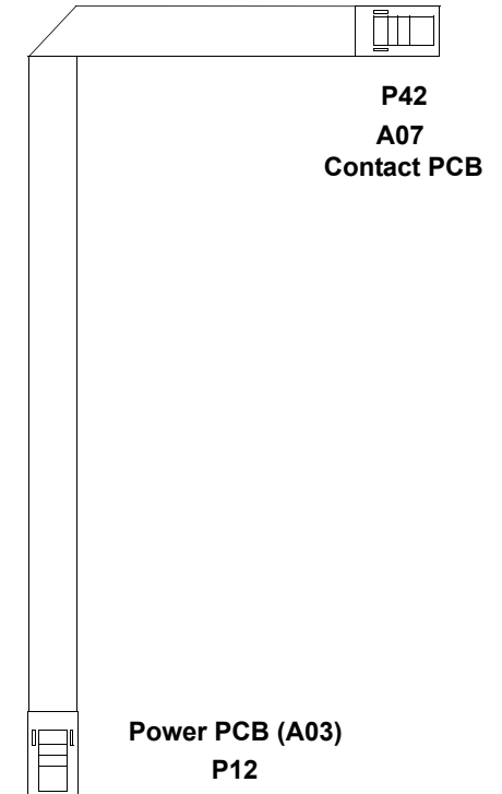
Figure 10.107—Power/contact PCB cable connections
