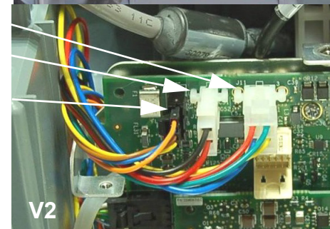
J11 connection (W10)
