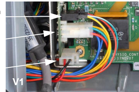
J13 connection (W10)
