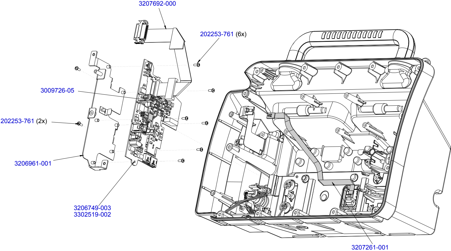
Figure 11.17—Rear Case view 4 of 7
