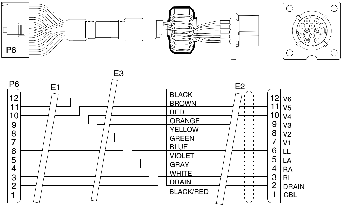
Figure 11.47—Diagram for item W07
