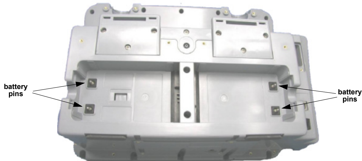
Figure 10.125—Battery pins
