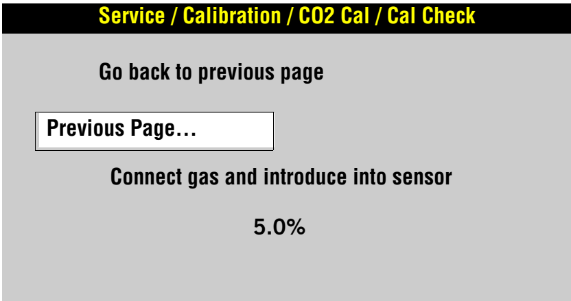
Figure 5.22—Service/Calibration submenu
