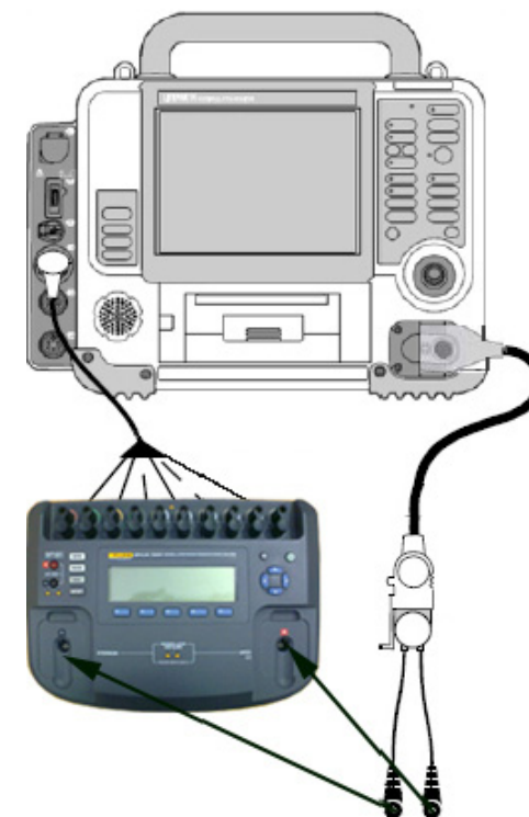
Figure 5.53—Pacer leads-off test setup
