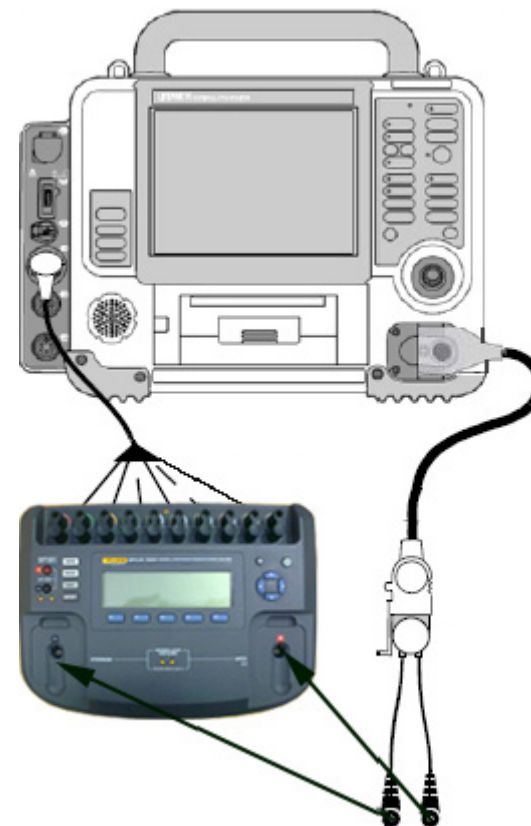
Figure 5.55—Pacer pulse width test setup
