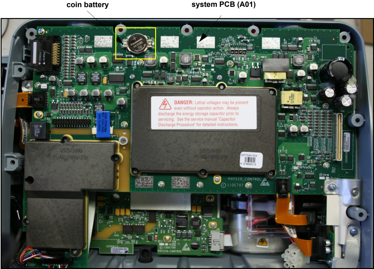
Figure 10.124—Coin battery location
