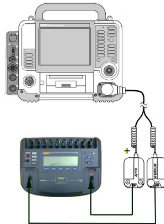
Figure 5.50—Standard paddles ECG characteristics test setup
