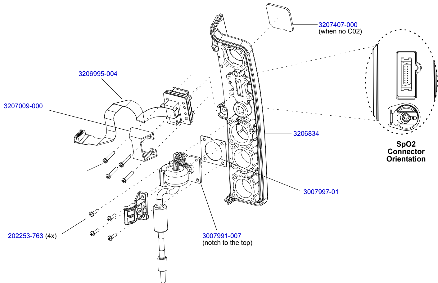
Figure 11.10—Parameter Bezel view 1 of 4 (ECG and optional SpO2)
