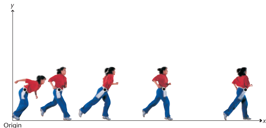
FIGURE 3-8 When the origin is at the left, the positive values of x extend horizontally to the right, and the positive values of y extend vertically upward.
