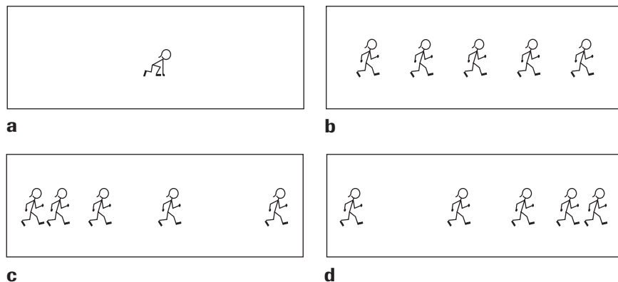
FIGURE 3-5 By noting the distance the jogger moves in equal time intervals, you can determine that the jogger in a is standing still, in b she is moving at a constant speed, in c she is speeding up, and in d she is slowing down.
