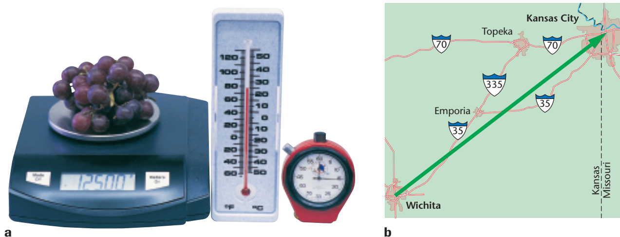
FIGURE 3-10 Time, temperature, and mass are scalar quantities, expressed as numbers with units. The arrow in b represents a vector quantity. It indicates the direction of Kansas City relative to Wichita and its length is proportional to the distance between the two cities.
