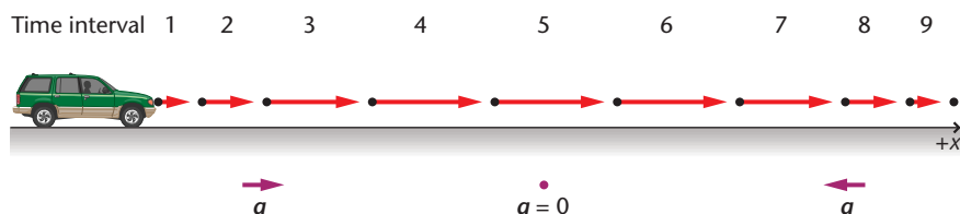
FIGURE 3–16 In this diagram, the origin is on the left. As a result, all the average velocity vectors are positive. The sign of the acceleration is determined by whether the car is speeding up or slowing down.
