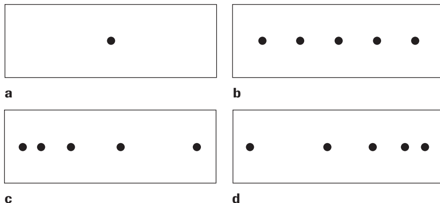
FIGURE 3–6 Using the particle model, you can draw simplified motion diagrams such as these for the jogger in Figure 3–5 .
