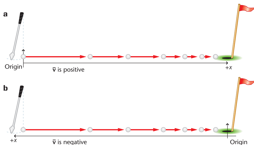
FIGURE 3–15 The sign of the average velocity depends upon the chosen coordinate system. The coordinate systems in a and b are equally correct.
