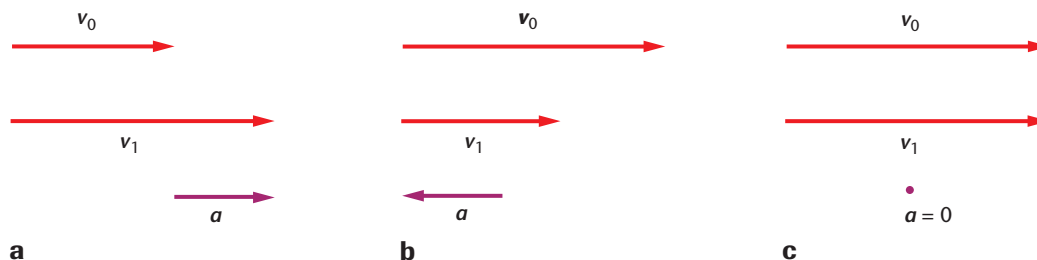
FIGURE 3-17 The direction of the acceleration is determined by whether the car is speeding up, slowing down, or traveling at constant speed.
