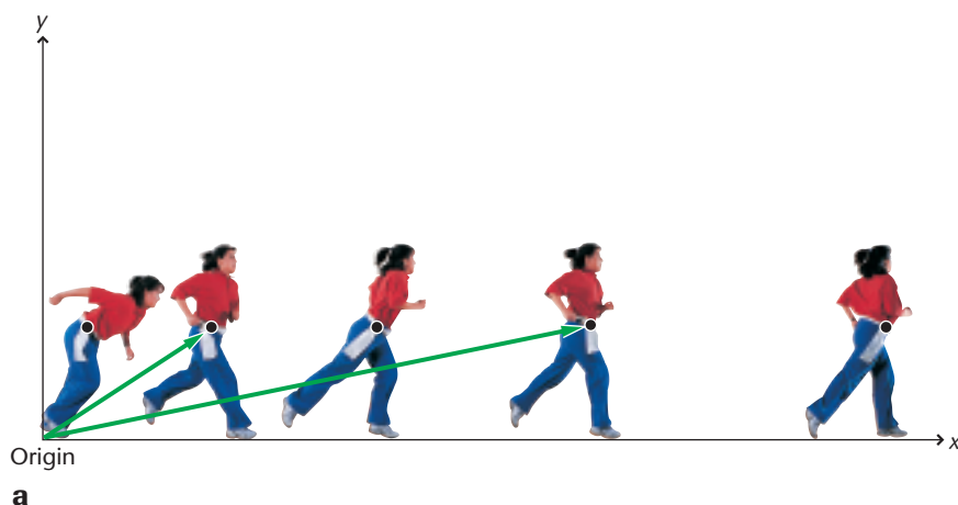
FIGURE 3–9 Two position vectors in a , drawn from the origin to the knot on the sprinter's belt, locate her position at two different times. The position of the sprinter in b , as she walks toward the starting block, is negative in this coordinate system.
