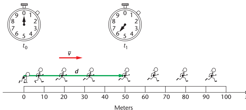
FIGURE 3–14 Average velocity vectors have the same direction as their corresponding displacement vectors. Their magnitudes are different but proportional and they have different units.
